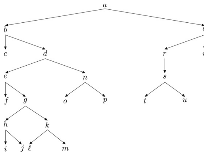
Fig. 2. The action of ADDCASE.
