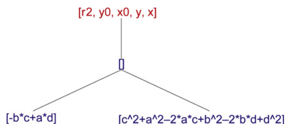
Fig. 5. Generic case for HT in the nine points circle Theorem.
