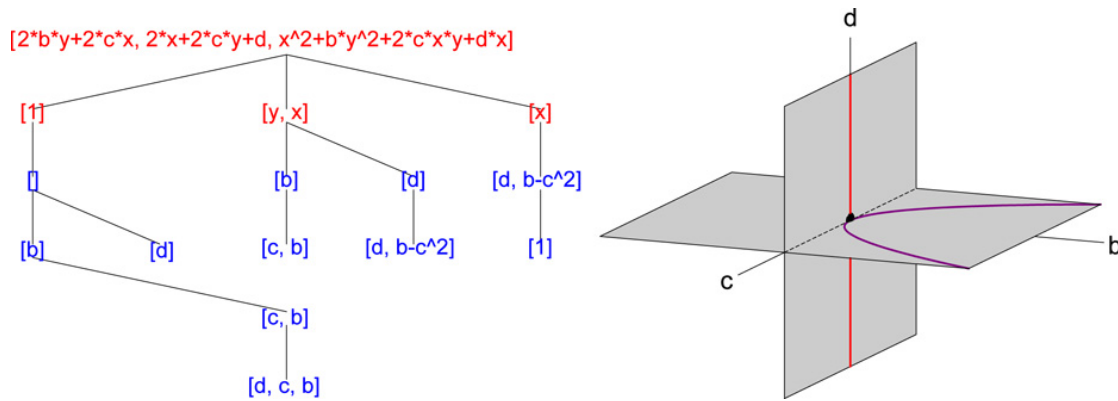
Fig. 3. Minimal canonical CGS for the singular points of a conic system.
