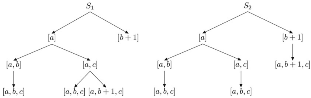
Fig. 1. Trees representing the sets S_1 and S_2 in generalized can-specification.
