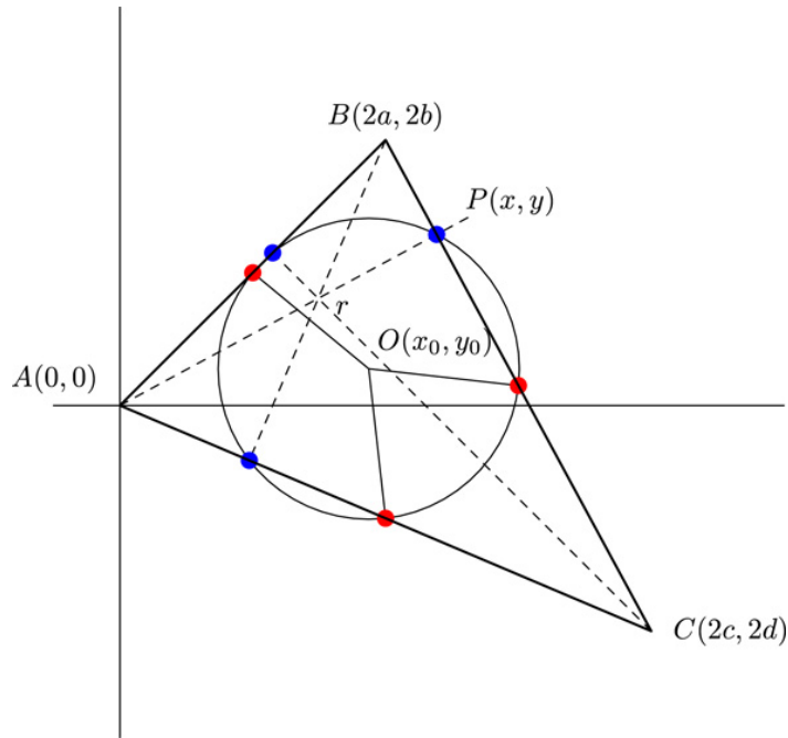
Fig. 4. Nine points circle Theorem.
